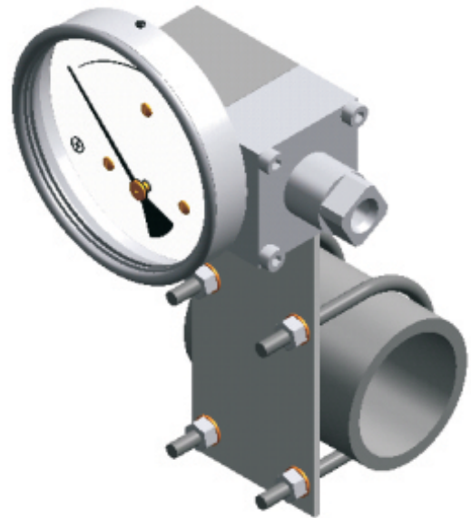
HORIZONTAL PIPE MOUNTING
