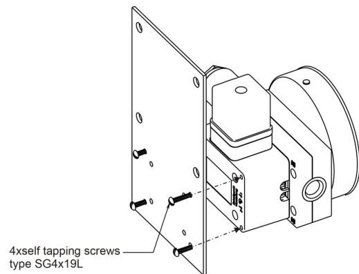
EXPLODED VIEW SHOWING FITMENT
