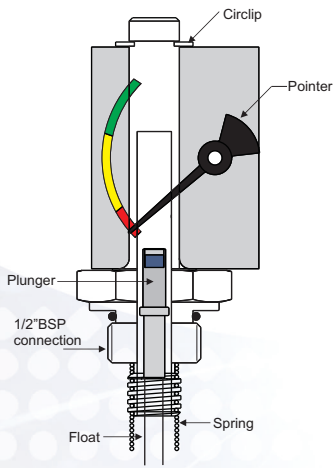
Gauge
